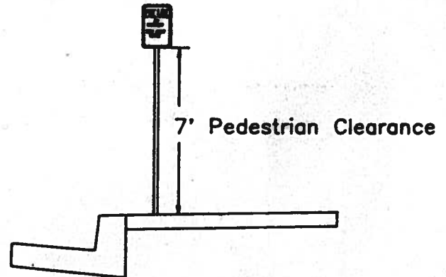
FIRE LANE Sign To Be Set Per City Standard ST10
